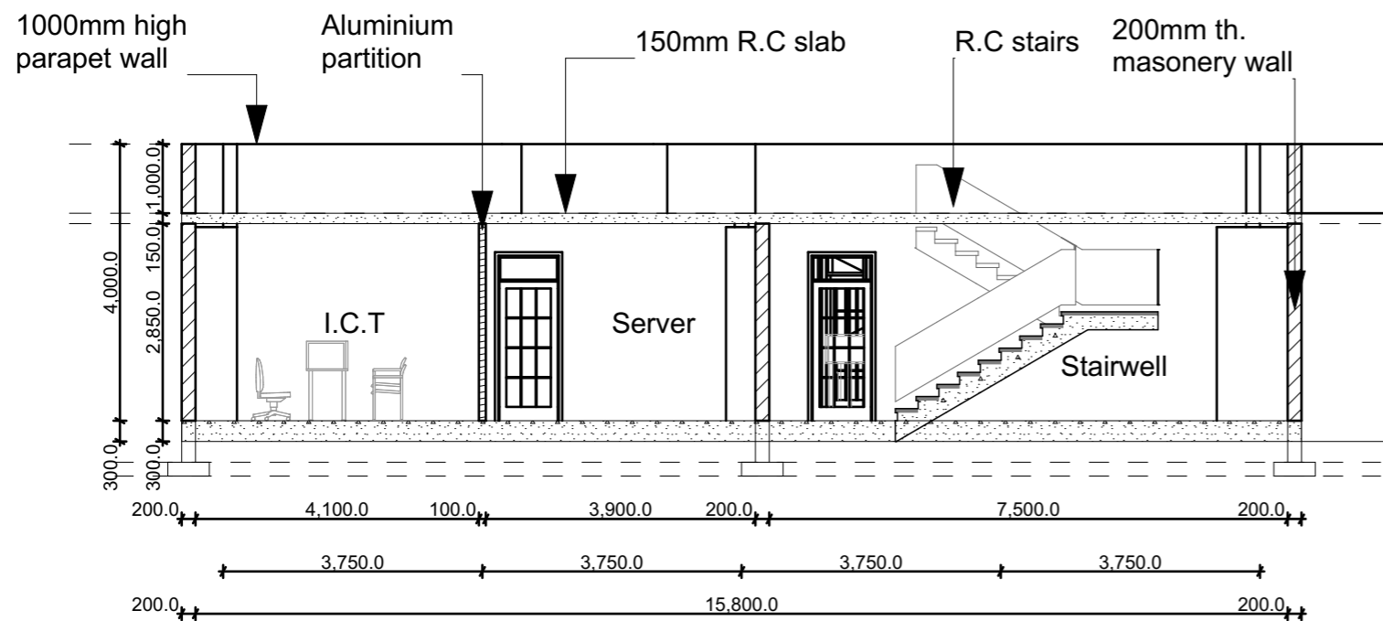
SECTION X-X 1:100
