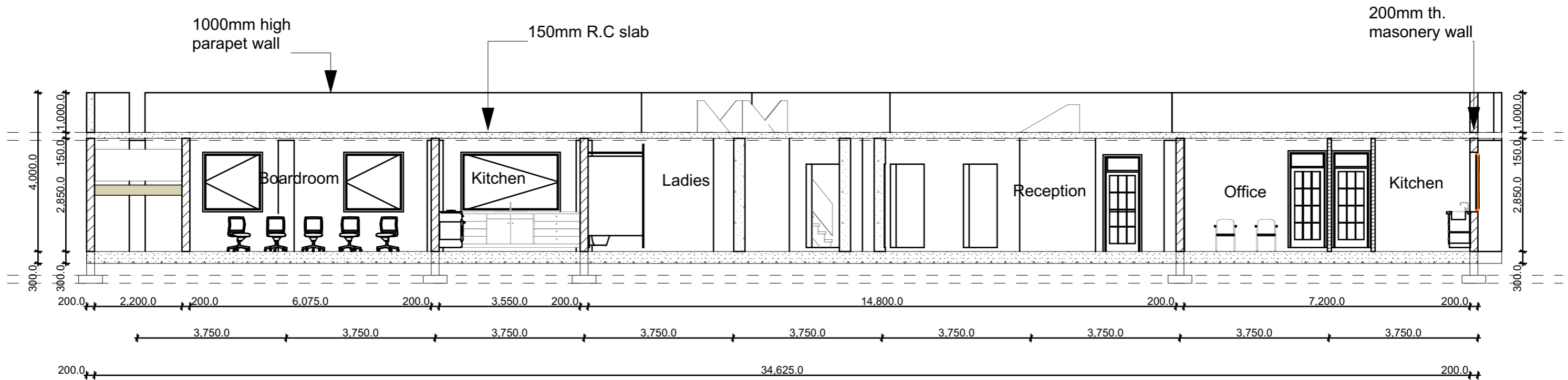
SECTION Y-Y 1:100
